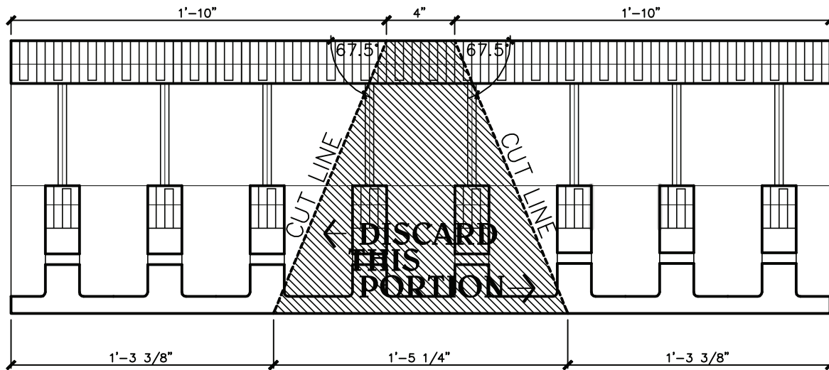
2 CUTTING DIAGRAM (TOP VIEW FULL BLOCK) SCALE: 1 1/2" = 1'-0"
