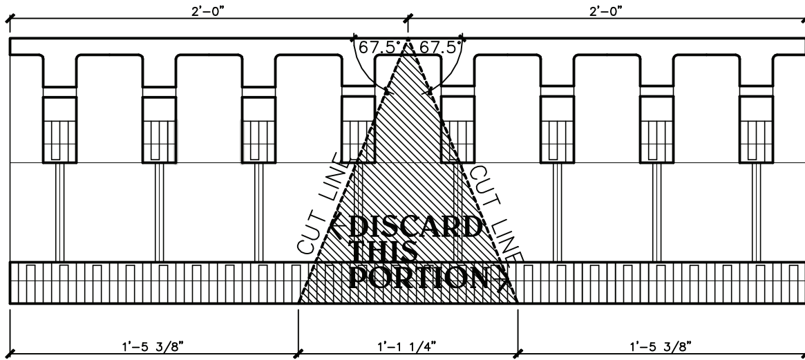
② CUTTING DIAGRAM (TOP VIEW FULL BLOCK) SCALE: 1 1/2" = 1'-0"
