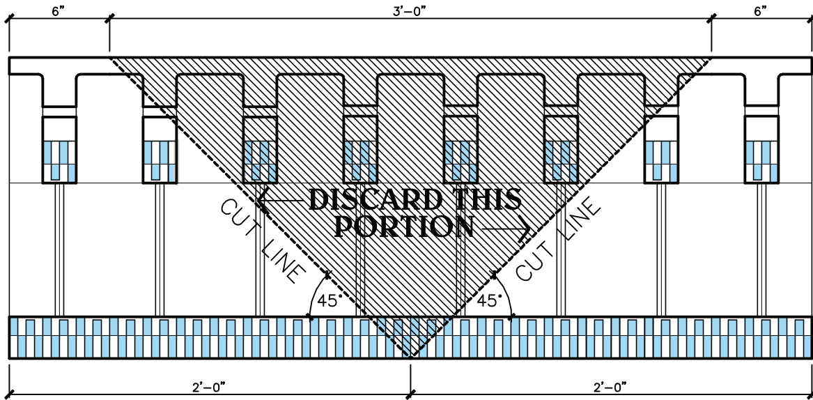
② CUTTING DIAGRAM (TOP VIEW FULL BLOCK) SCALE: 1 1/2" = 1'-0"
