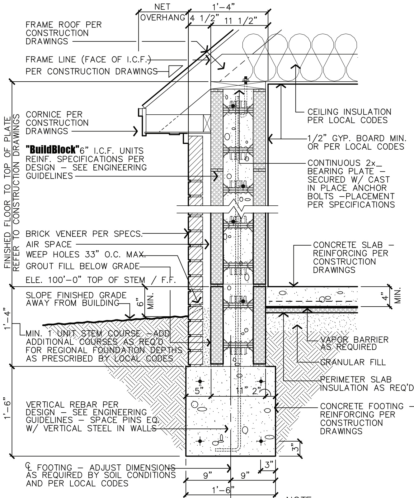
1 06 TYPICAL WALL SECTION SCALE: 1" = 1'-0"
