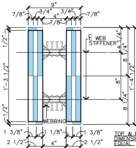
1 SIDE VIEW 01a SCALE: 1 1/2" = 1'-0"
