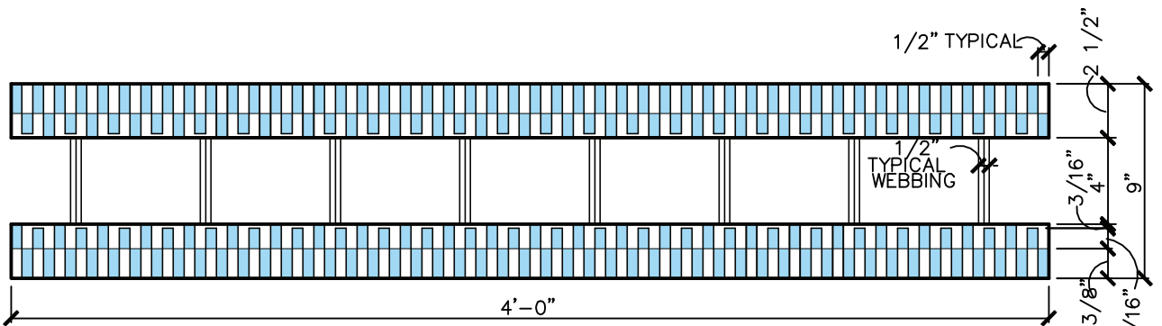
2 TOP / BOTTOM VIEW (REVERSIBLE) 01a SCALE: 1 1/2" = 1'-0"
