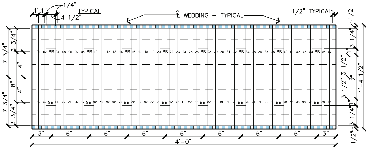
3 FRONT VIEW 01a SCALE: 1 1/2" = 1'-0"
