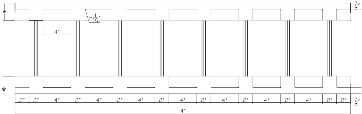
2 / 03 TOP / BOTTOM VIEW (REVERSIBLE) SCALE: 1 1/2" = 1'-0"
