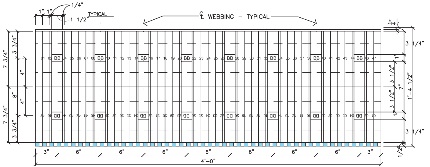
3 / 03 FRONT VIEW SCALE: 1 1/2" = 1'-0"
