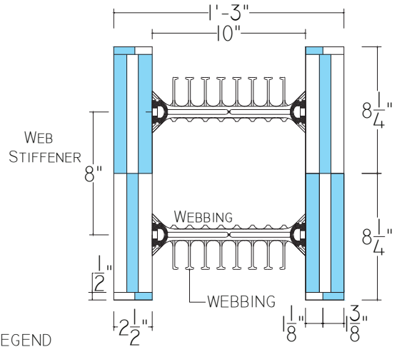
1 01 SIDE VIEW SCALE: NTS
