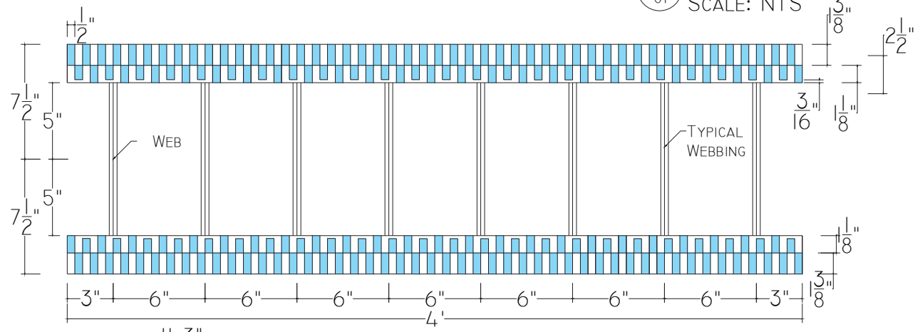
2 01 TOP / BOTTOM VIEW (REVERSIBLE) SCALE: NTS
