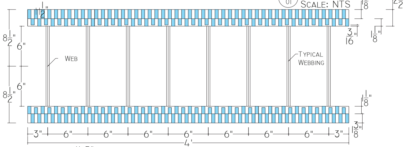
2 TOP / BOTTOM VIEW 01 (REVERSIBLE) SCALE: NTS
