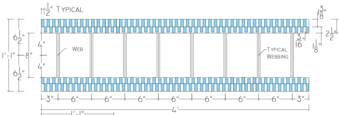
2 01 TOP / BOTTOM VIEW (REVERSIBLE) SCALE: NTS
