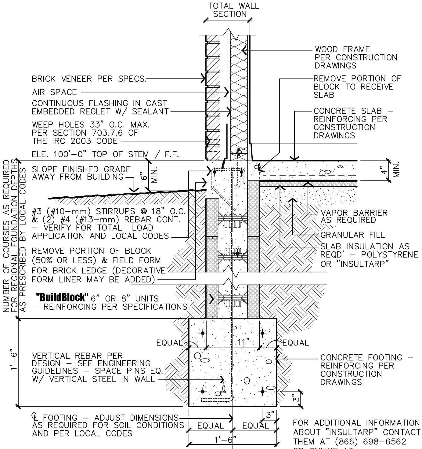
1 FOUNDATION DETAIL 09 SCALE: 1" = 1'-0"
