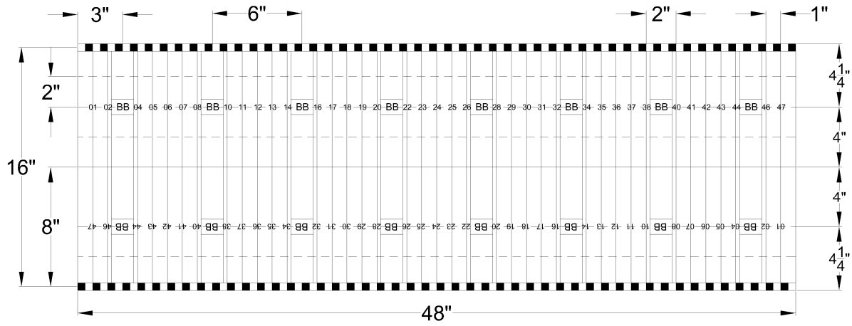
3 FRONT VIEW
