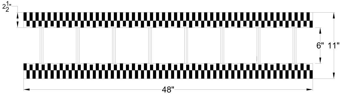
2 TOP/BOTTOM VIEW (REVERSIBLE)
