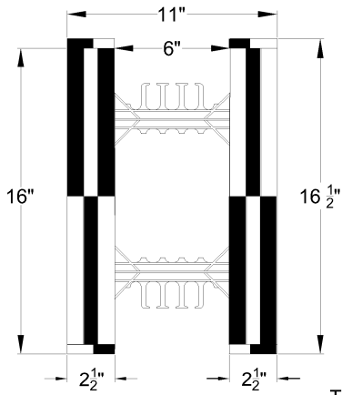
1 SIDE VIEW
