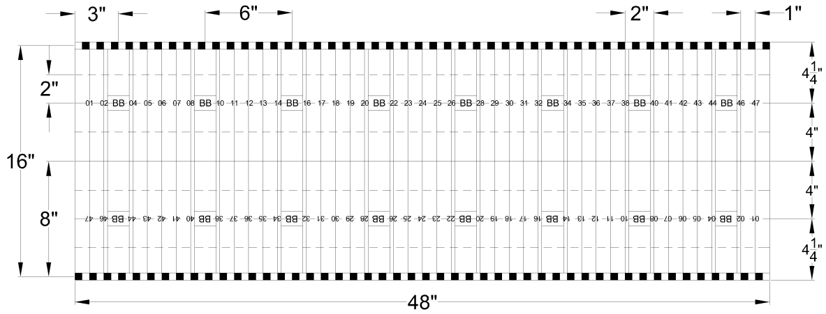
3 FRONT VIEW
