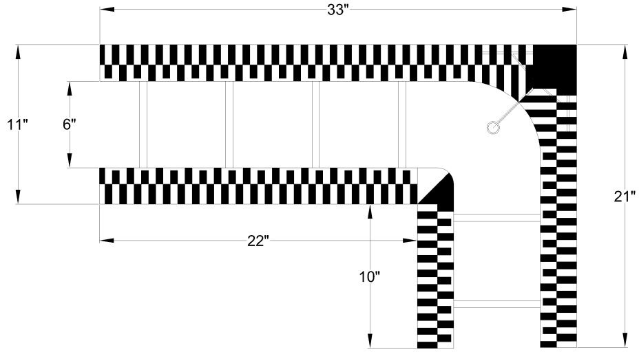
2 TOP/BOTTOM VIEW (90° REVERSIBLE)
