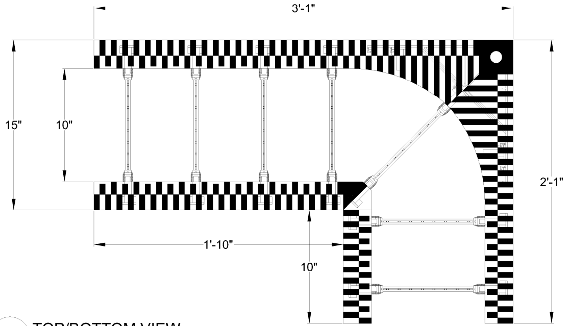
2 TOP/BOTTOM VIEW (90° REVERSIBLE)
