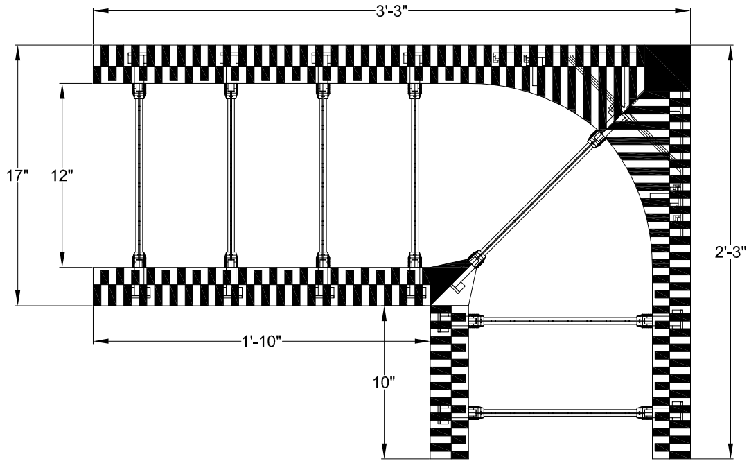
2 TOP/BOTTOM VIEW (90° REVERSIBLE)
