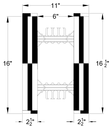
1 SIDE VIEW
