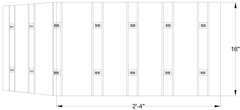
3 OUTSIDE VIEW
