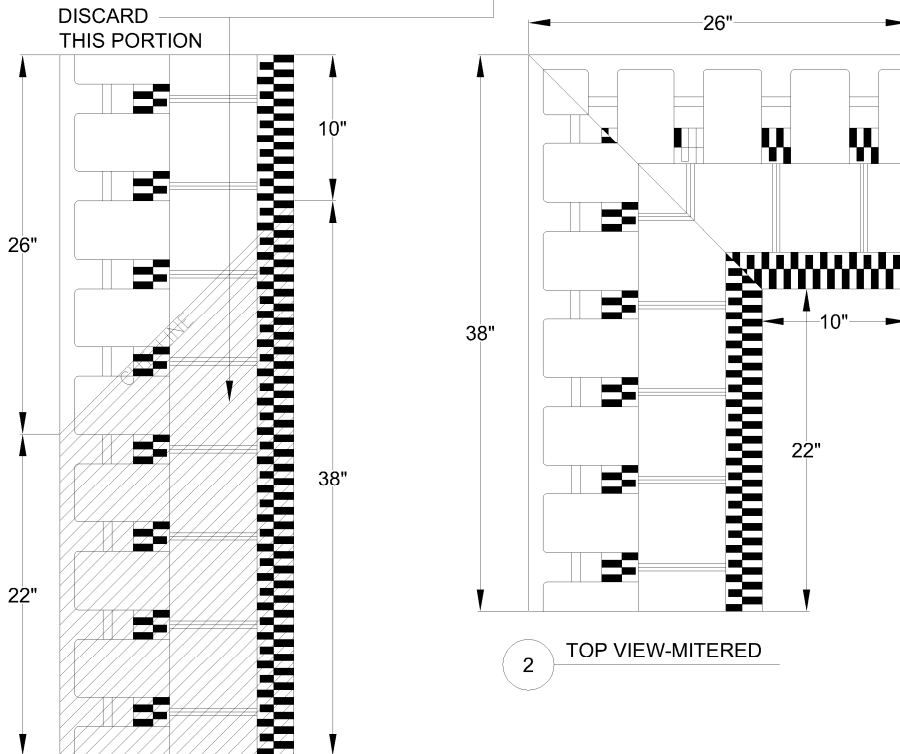
1 CUTTING DIAGRAM (TOP VIEW FULL BLOCK)
