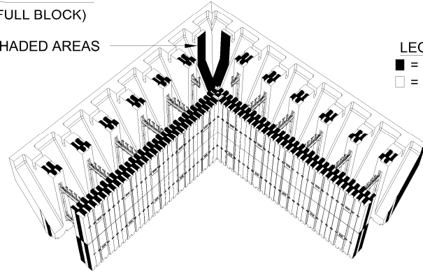
3 ISOMETRIC VIEW
