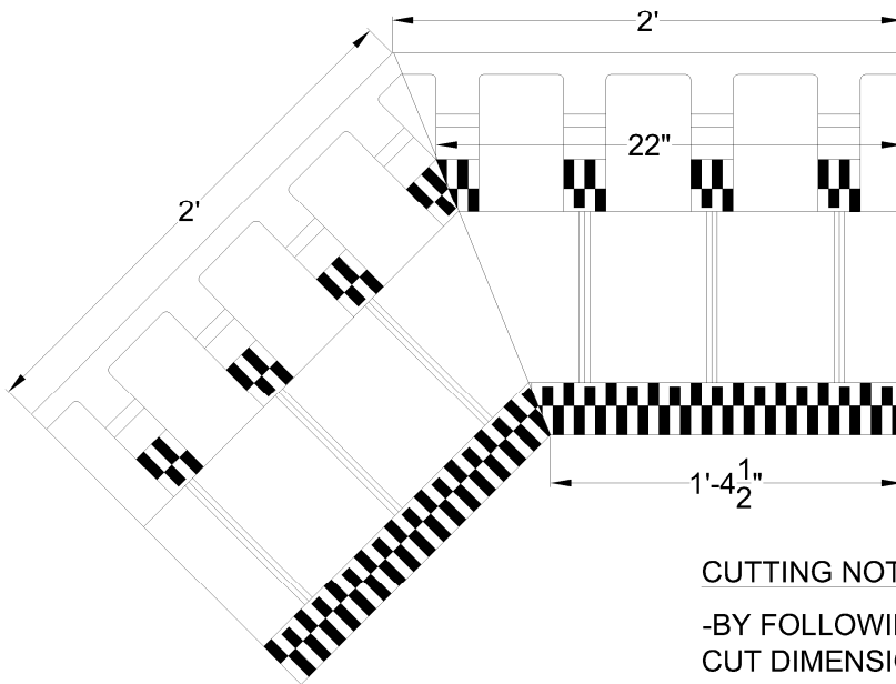
2 TOP VIEW-MITERED
