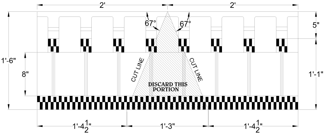
1 CUTTING DIAGRAM (TOP VIEW FULL BLOCK)
