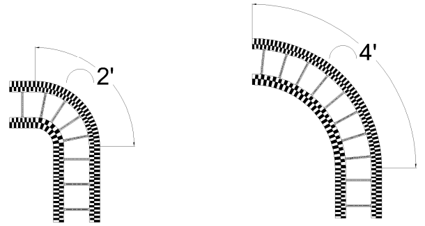
1 BR0602-TOP VIEW
