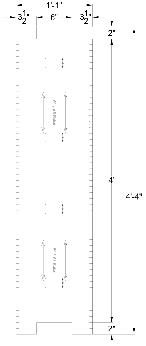
3 BOTTOM VIEW
