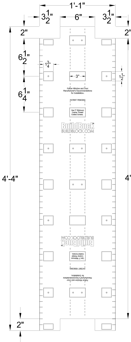
1 TOP VIEW
