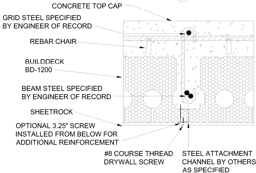
3 SIDE VIEWS
