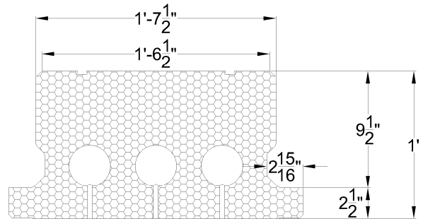
2 BOTTOM VIEW
