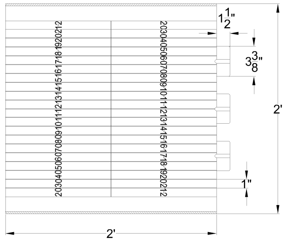
2 BOTTOM VIEW
