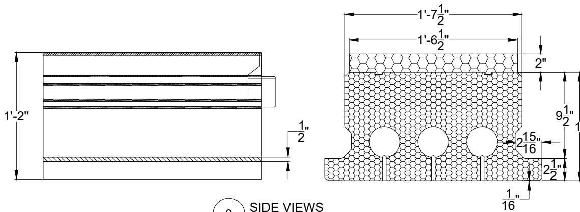
3 SIDE VIEWS
