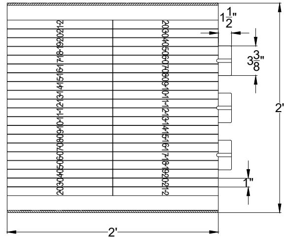
2 BOTTOM VIEW
