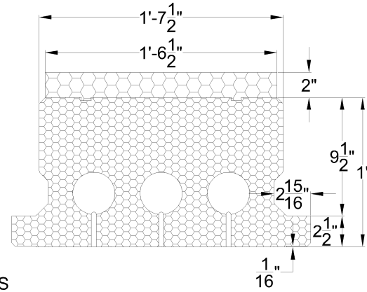
2 BOTTOM VIEW
