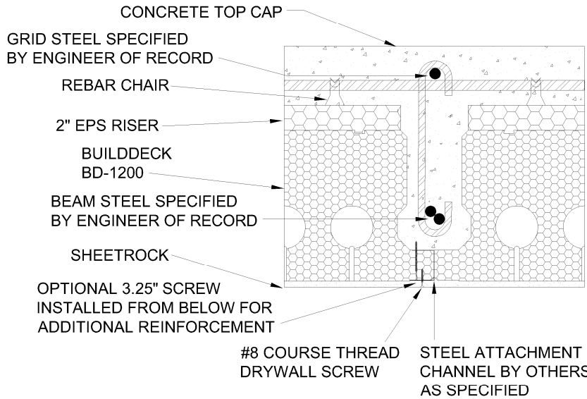
3 SIDE VIEWS
