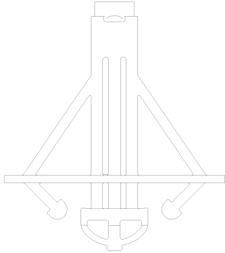
1 FRONT VIEW WITHOUT CAP
