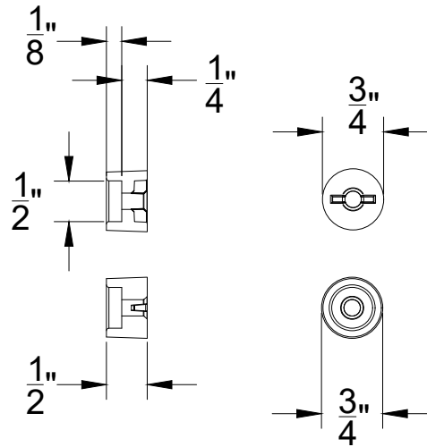
4 CAP VIEWS
