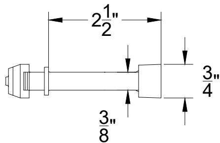
5 BOTTOM VIEW
