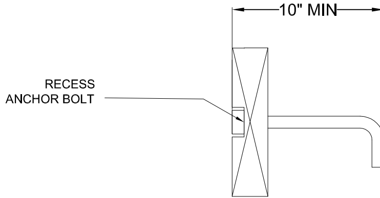
DETAIL OF NOTCHED WOOD PLATE AND ANCHOR BOLT NOT TO SCALE
