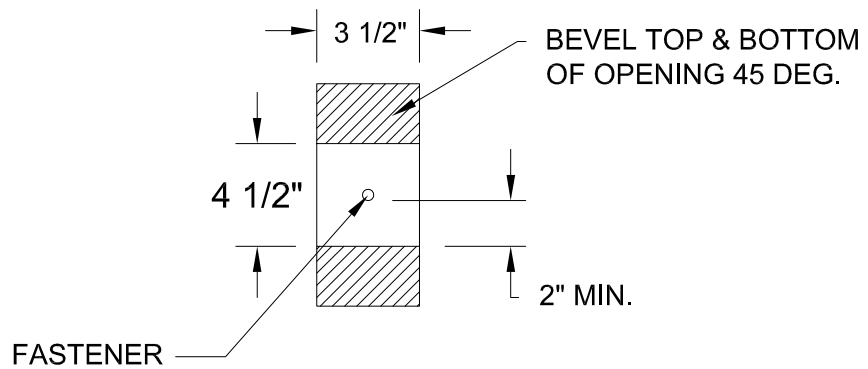
TYP. FORM CUTOUT
