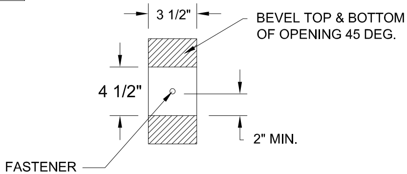
TYP. FORM CUTOUT
