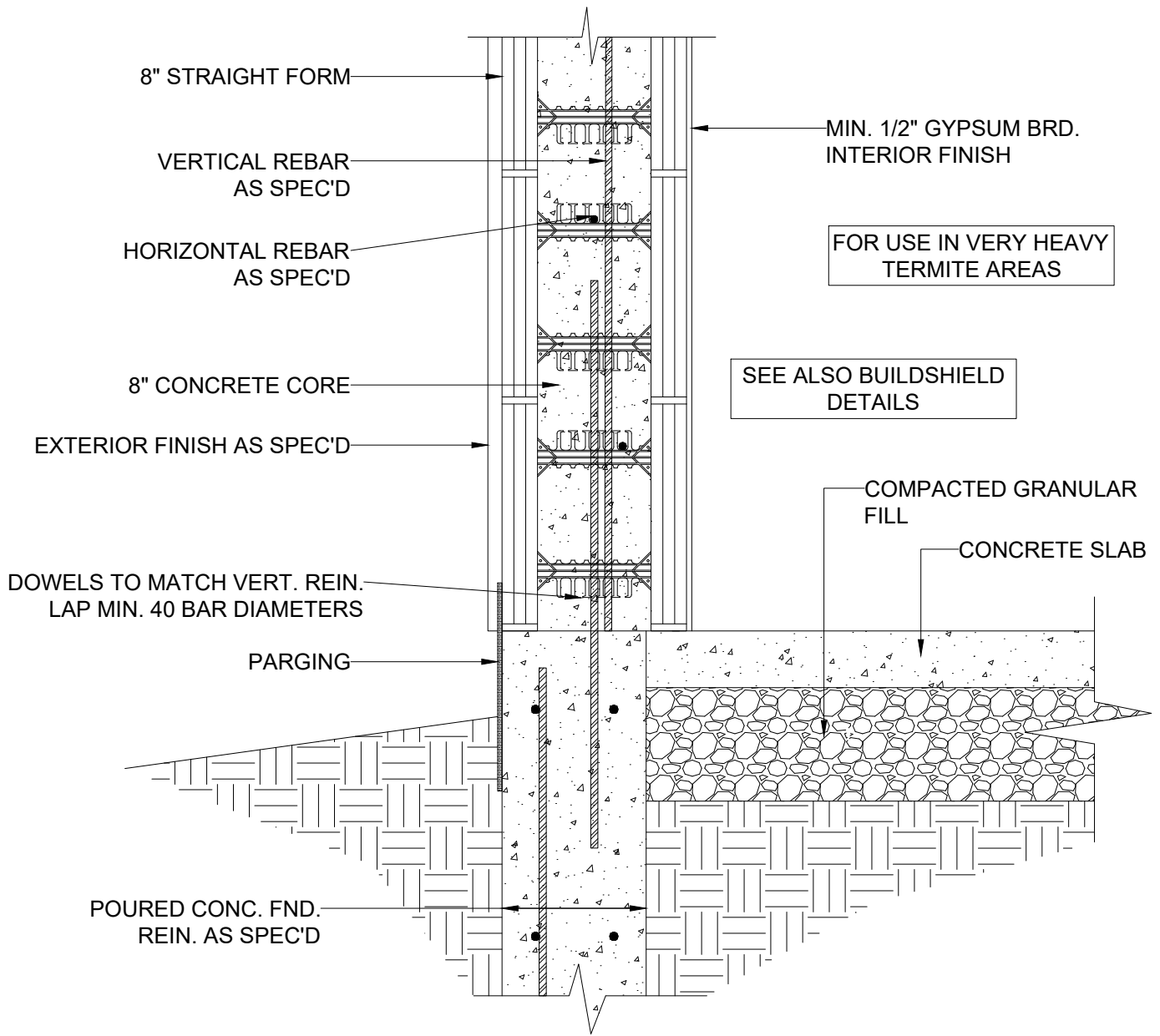
1 CONCRETE STEM WALL ABOVE GRADE 8 INCH
