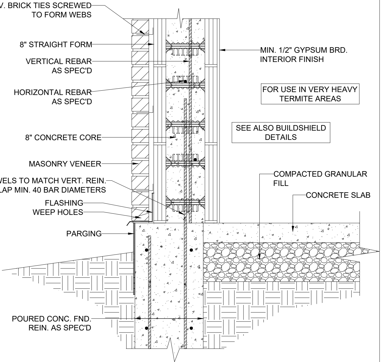
1 CONCRETE STEM WALL ABOVE GRADE 8 INCH
