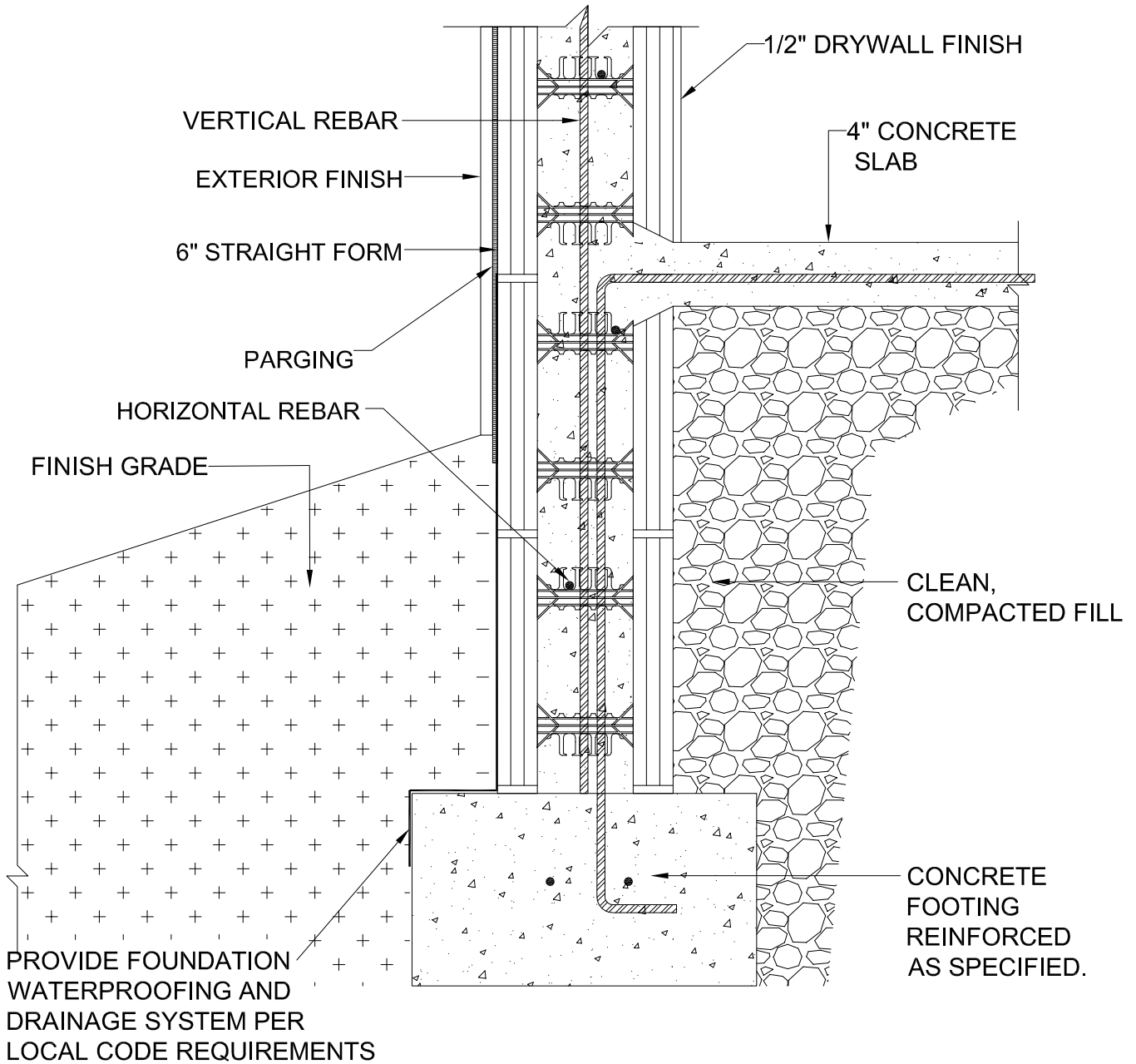
1 SLAB INTO STEM WALL 6 INCH
