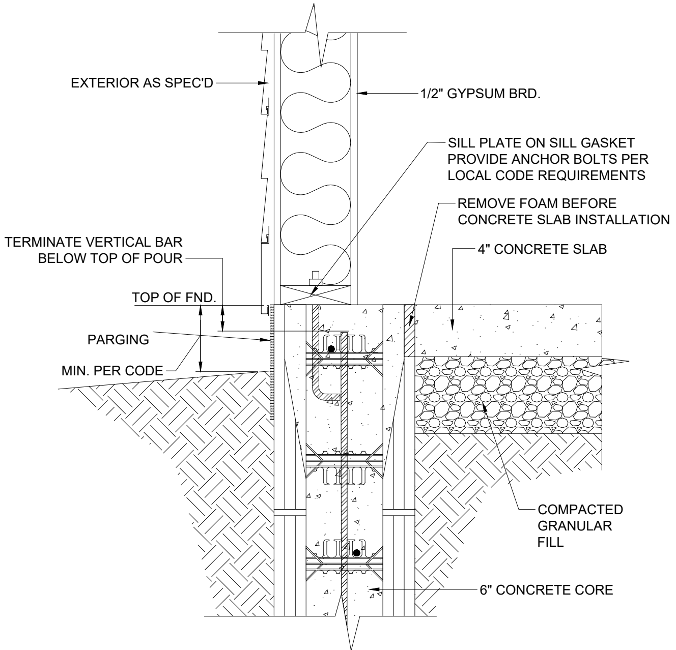
1 FROST WALL INTERIOR SLAB ON GRADE 6" FORM
