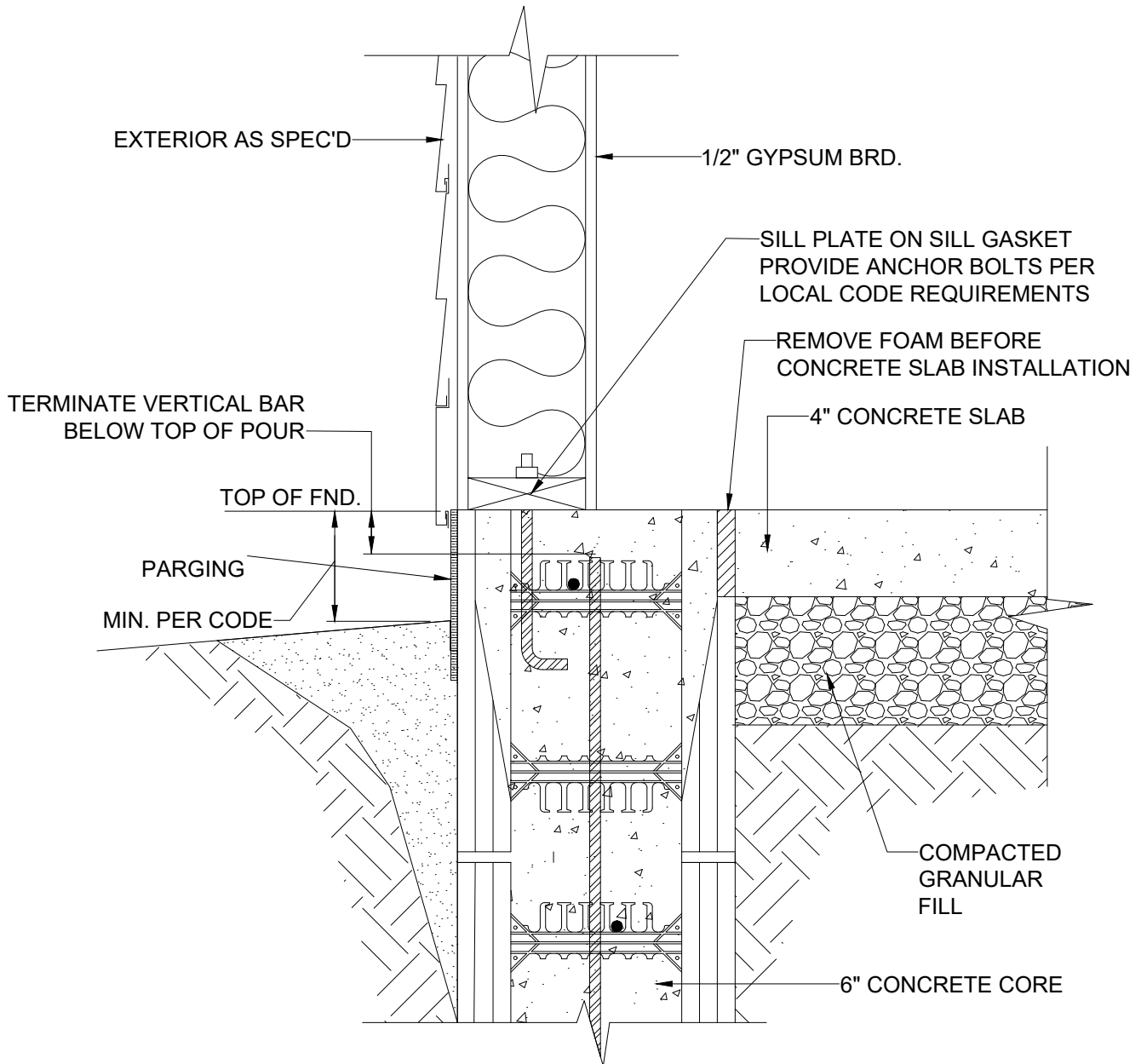
1 FROST WALL INTERIOR SLAB ON GRADE 8" FORM
