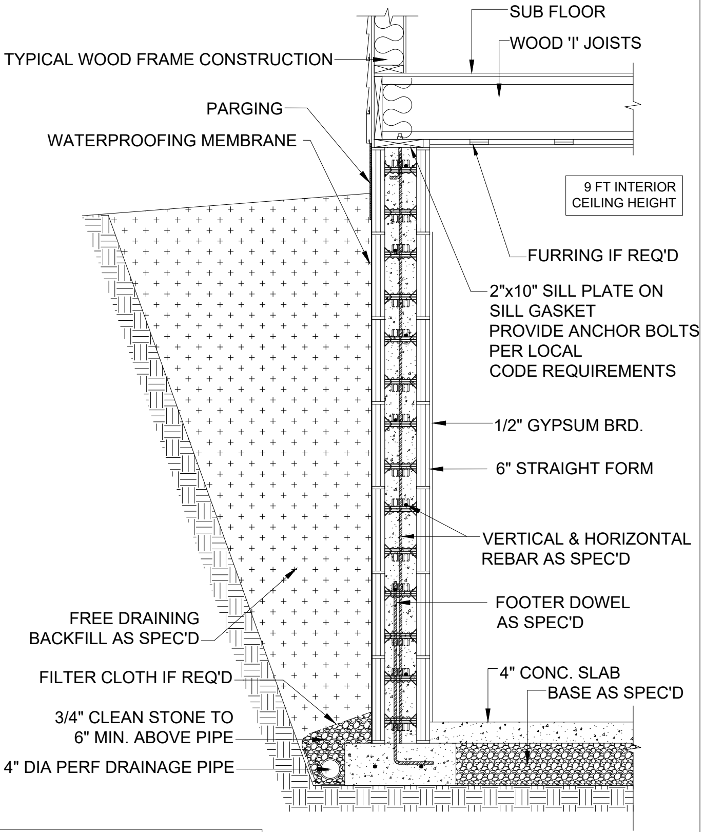
TYPICAL FOUNDATION 9' HIGH
