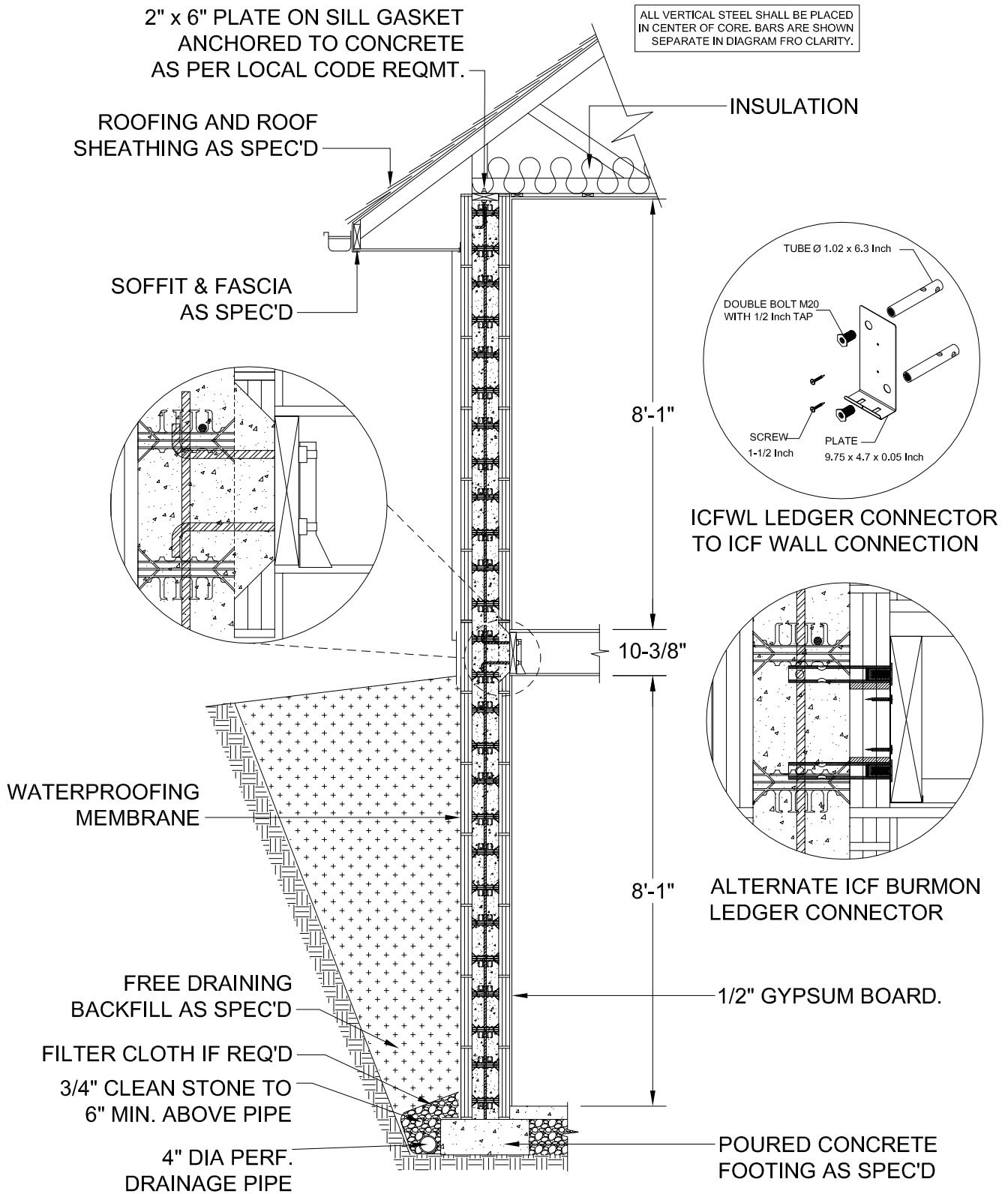
1 WALL SECTION 1 STORY ABOVE GRADE 6 INCH
