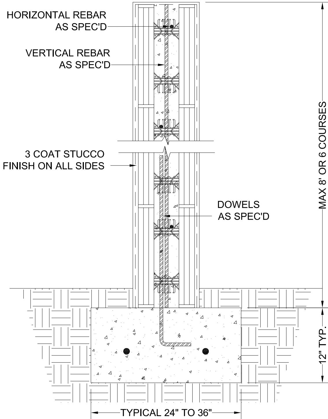
○ TYPICAL PROPERTY LINE WALL 4 INCH
