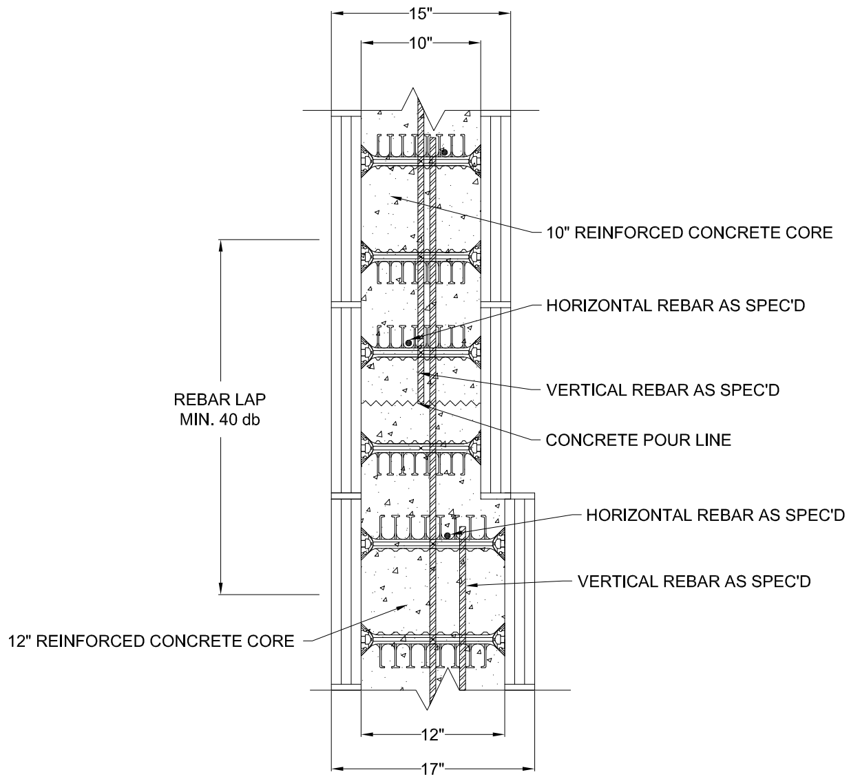
1 12" FORM TO 10" FORM TRANSITION ABOVE GRADE 12 INCH TO 10 INCH
