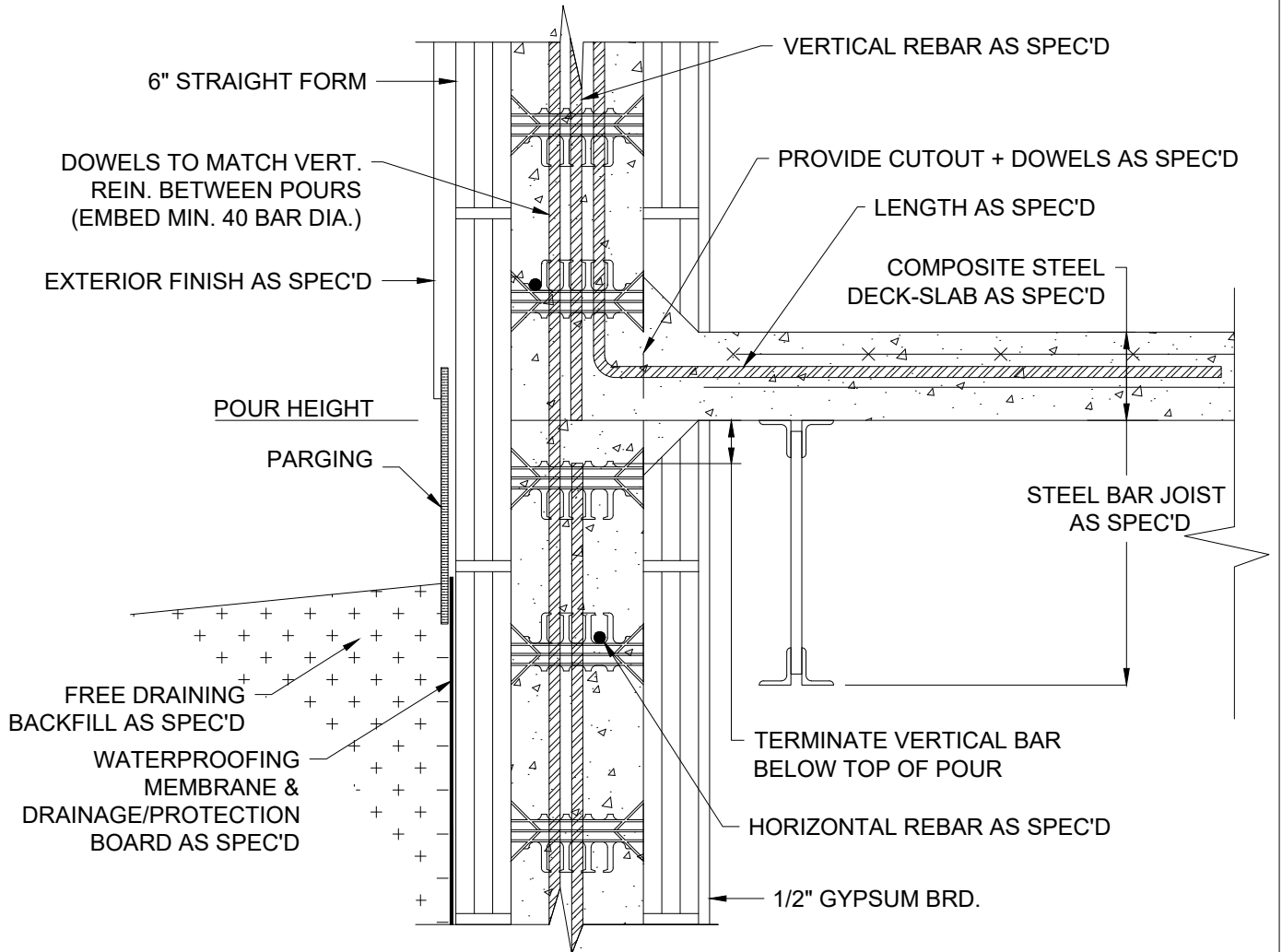
1 COMPOSITE STEEL DECK SLAB WITH STEEL JOIST 6 INCH
