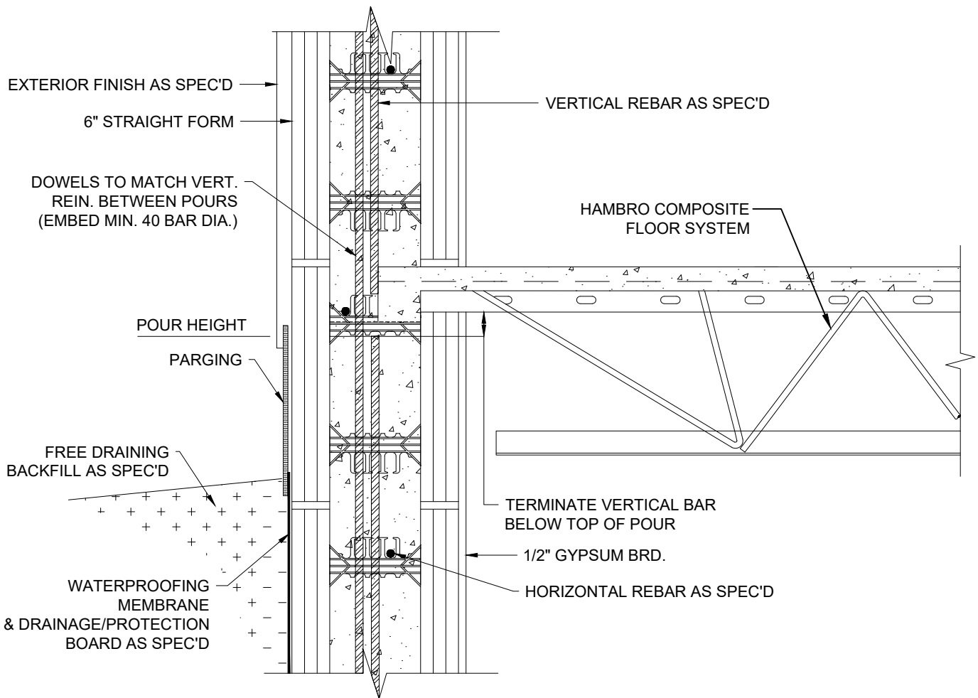
1 HAMBRO COMPOSITE FLOOR SYSTEM 6 INCH
