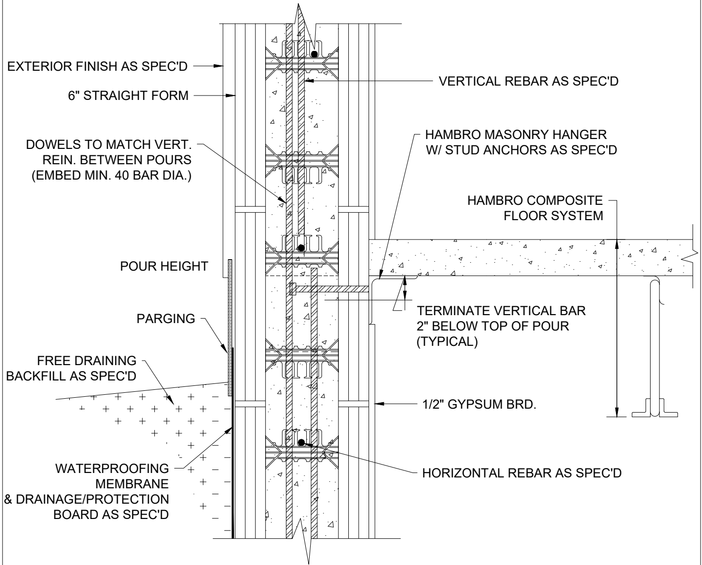
1 HAMBRO COMPOSITE FLOOR SYSTEM 6 INCH
