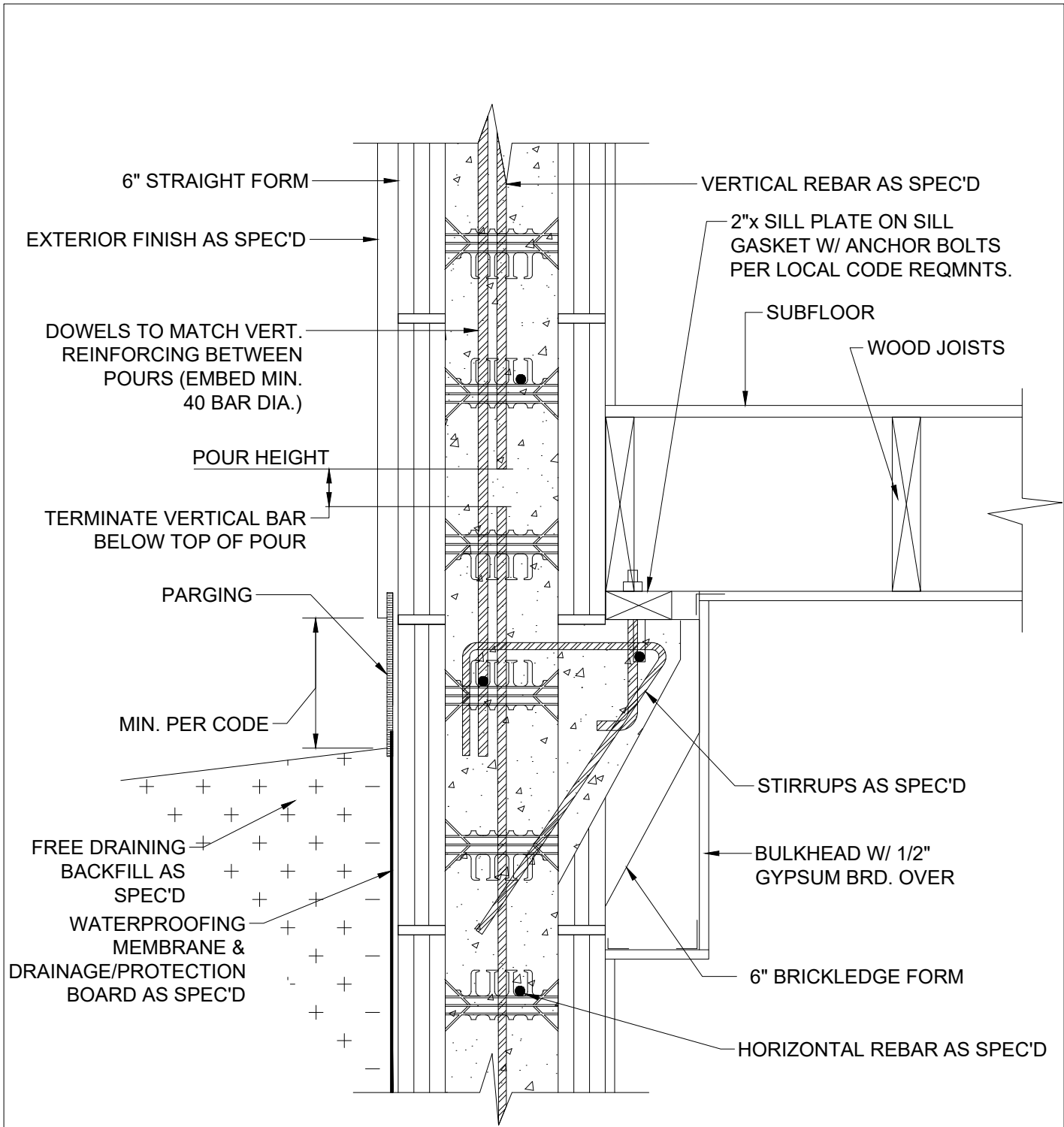
1 JOISTS ON EXTENDED FORM 6 INCH
