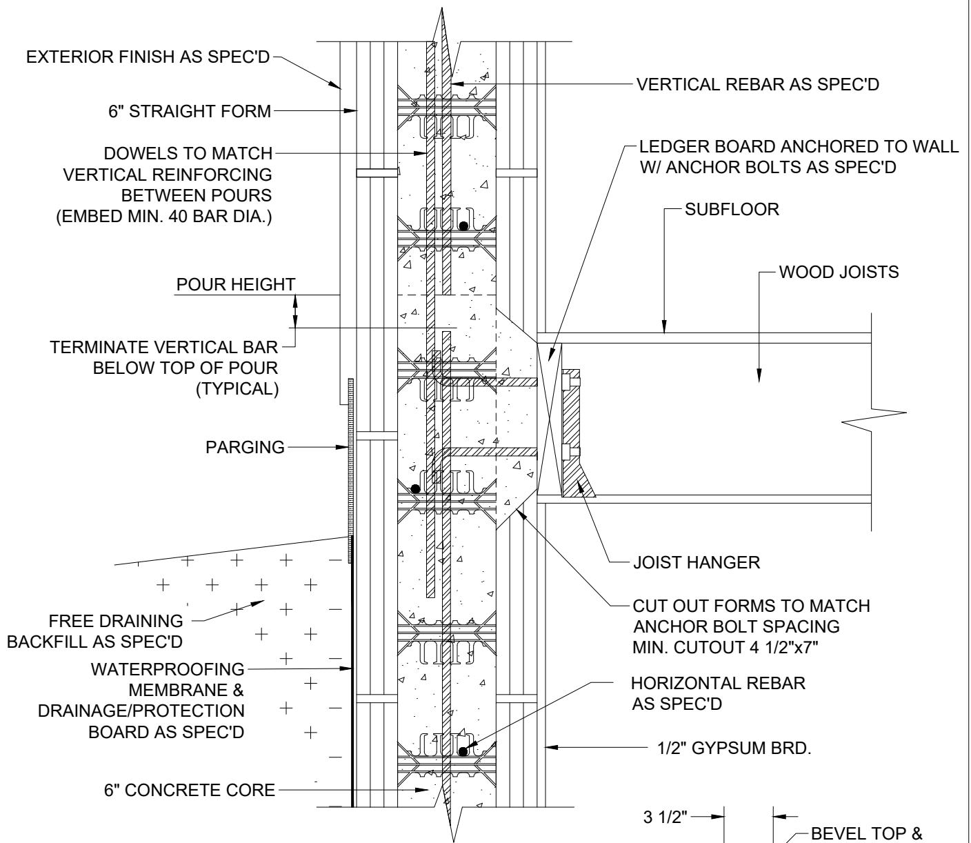
1 LEDGER BOARD CONNECTION 6 INCH
