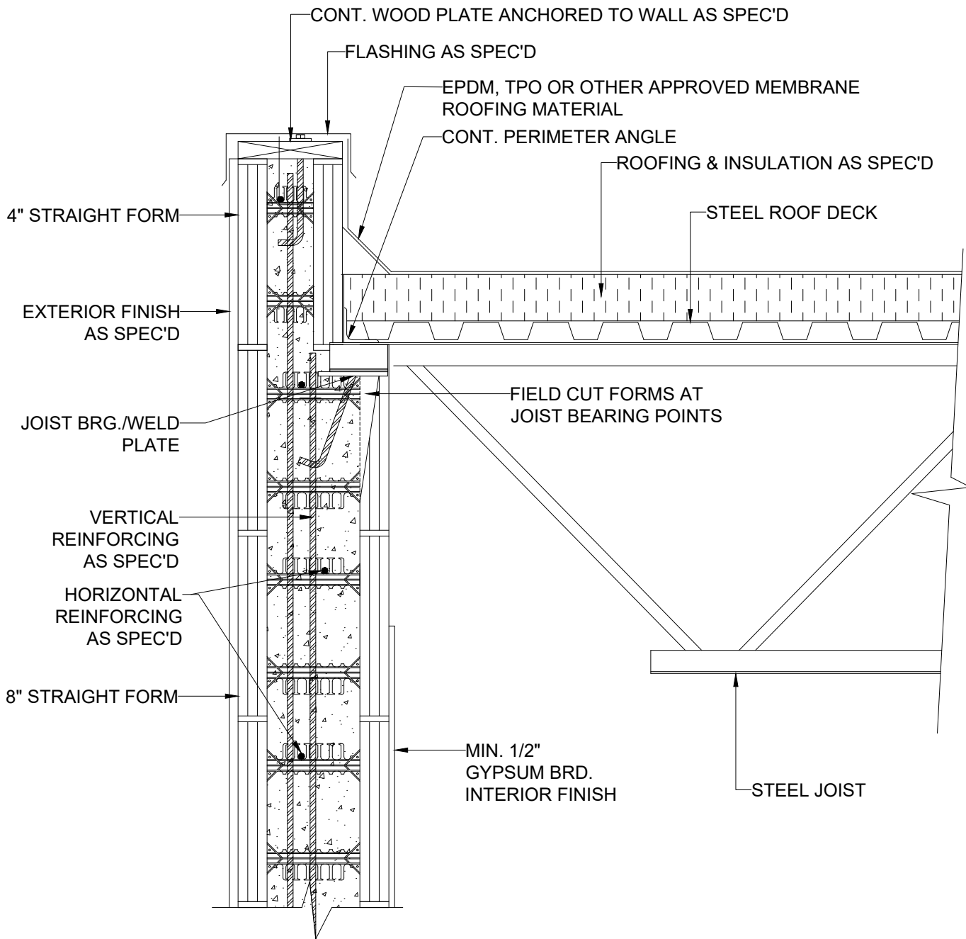
1 STEEL JOIST ROOF DETAIL BEARING WALL WITH PARAPET 8 INCH TO 4 INCH
