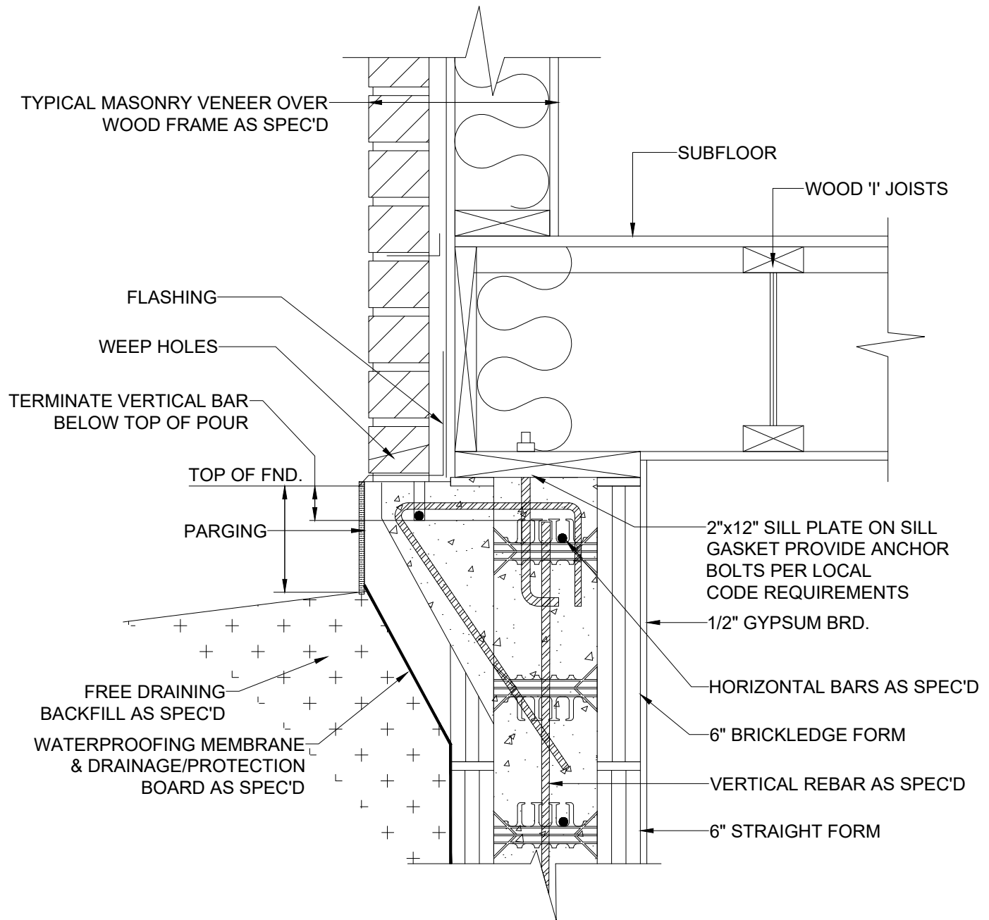
1 SILL PLATE DETAIL 6" INCH
