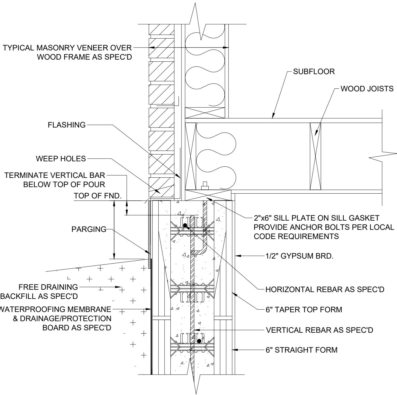
1 SILL PLATE DETAIL 6" INCH
