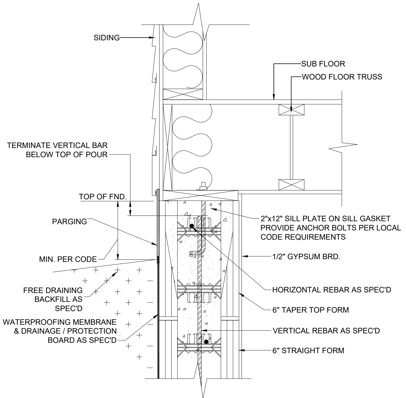
1 SILL PLATE DETAIL 6 INCH
