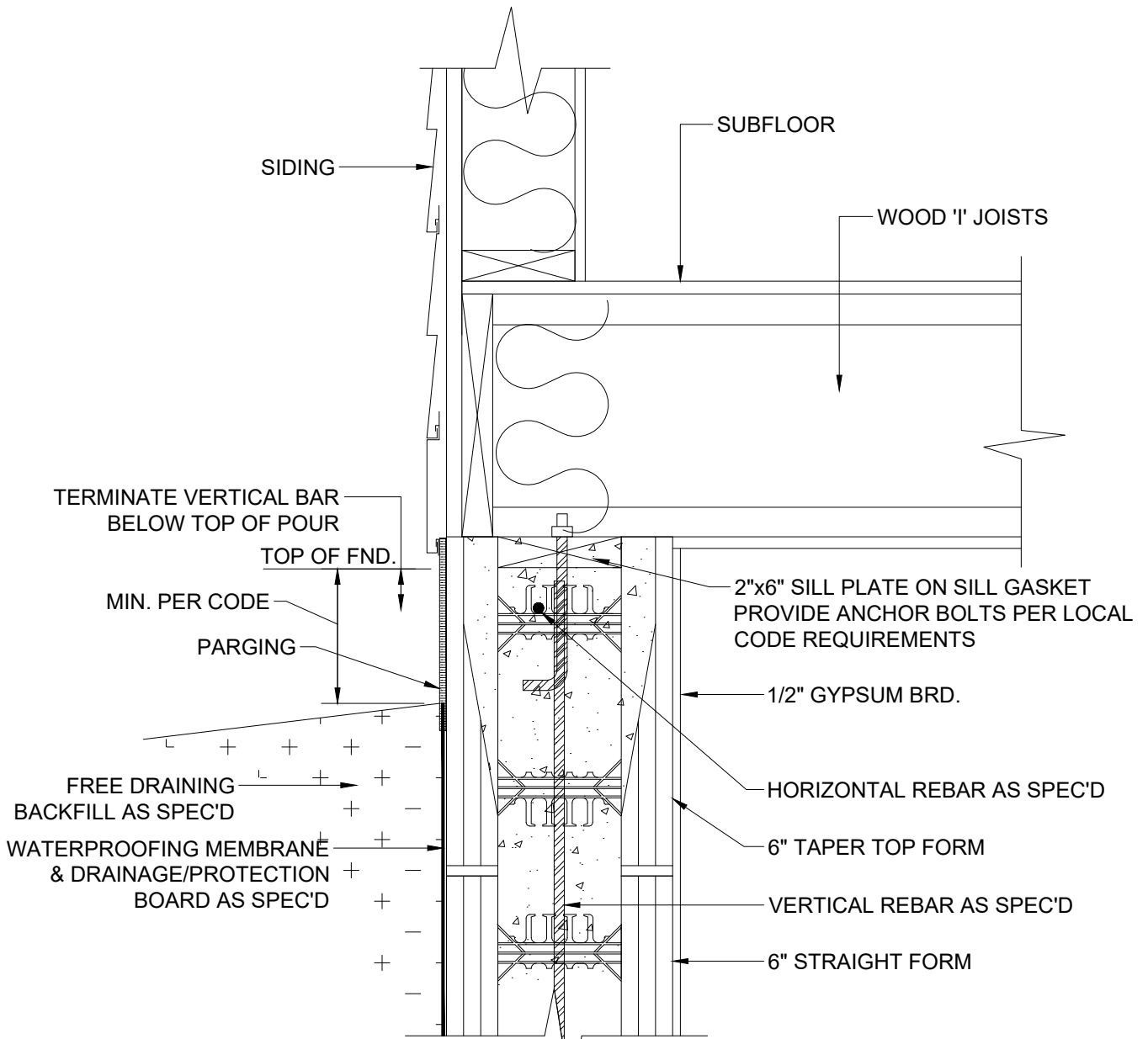
1 SILL PLATE DETAIL 6 INCH
