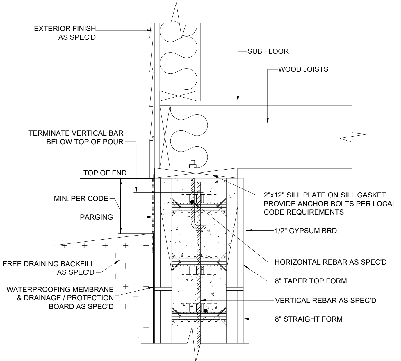
1 SILL PLATE DETAIL 8 INCH
