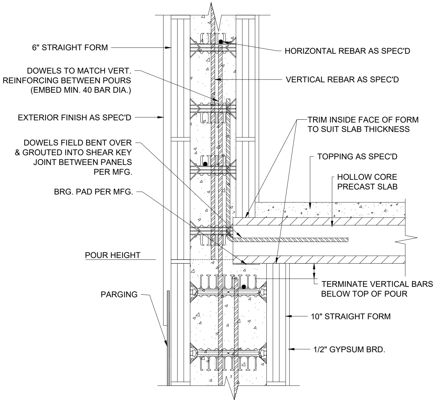
1 HOLLOW CORE PRECAST FLOOR SLAB 10 INCH TO 6 INCH
