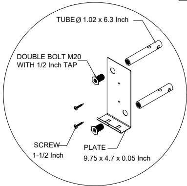
ICFWL LEDGER CONNECTOR TO ICF WALL CONNECTION
