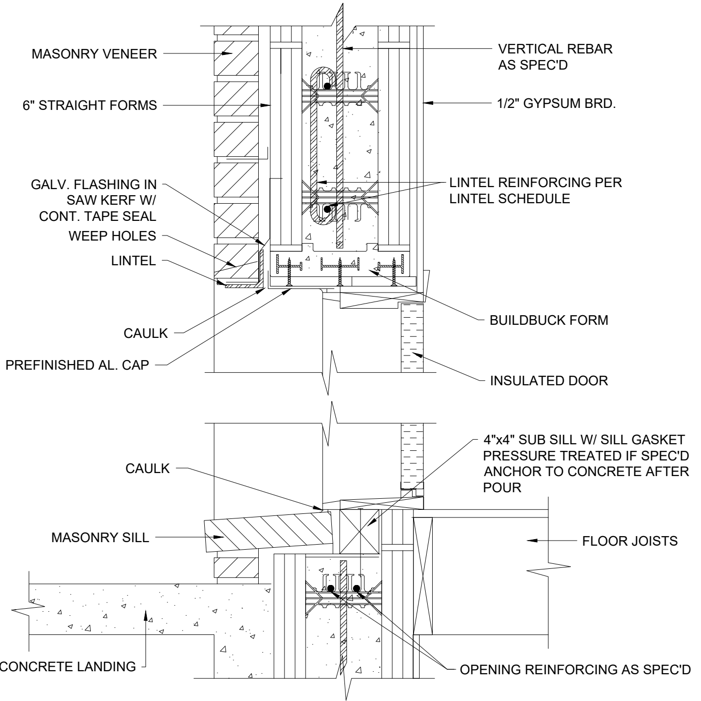
1 DOOR HEAD/SILL DETAIL 6 INCH
